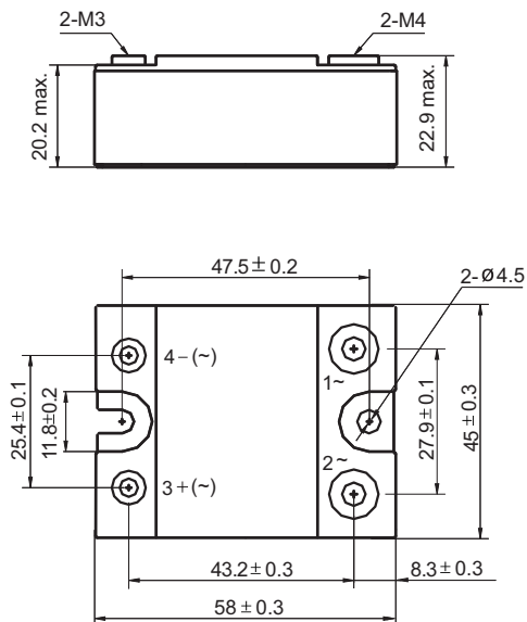
Outline Dimensions
