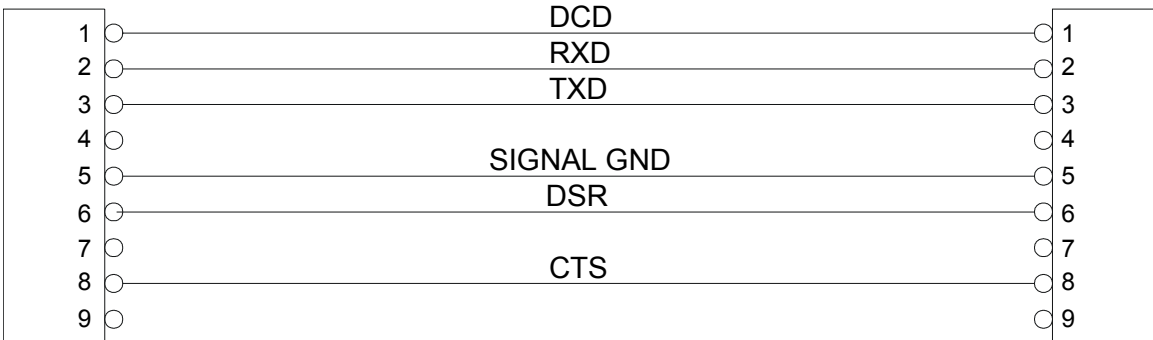
9-pin connector (s'print cable)
